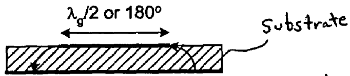
Figure 1: Patch antenna (Prior Art)
