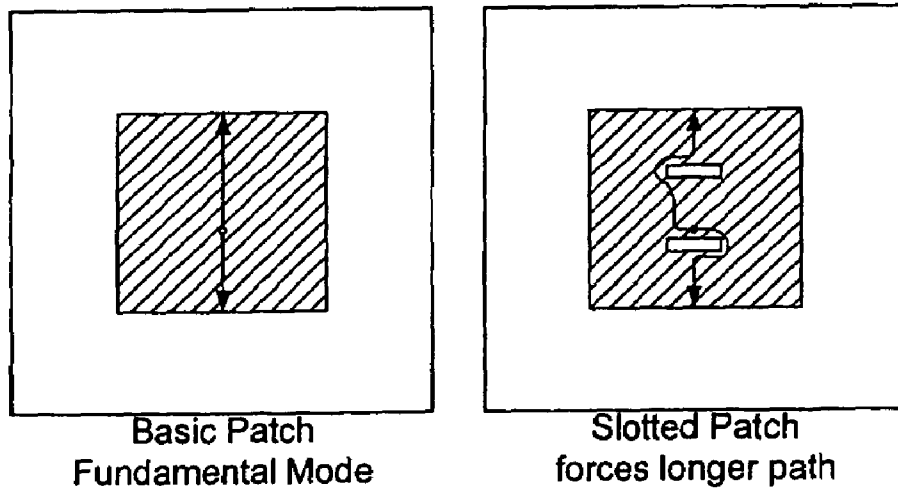
Figure 3: Basic Patch Vs. Slotted Patch (Prior Art)
